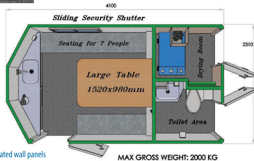
INTERNAL LAYOUT FLOOR PLAN
